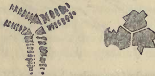
FIG. 3.—Last remains of spicules ( \times 1000 ) of Guancha coriacea , decalcified slowly in glycerin.
